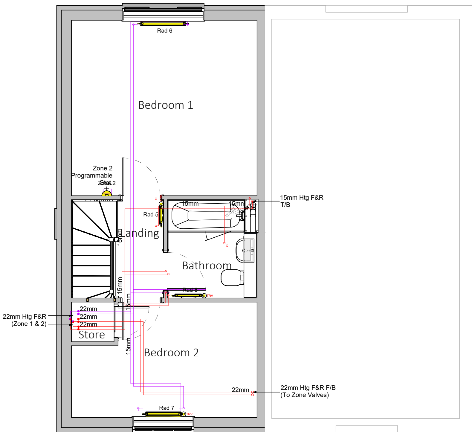
1 First Floor Heating GA 1 : 50
